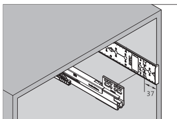
Double-wall Drawer System
