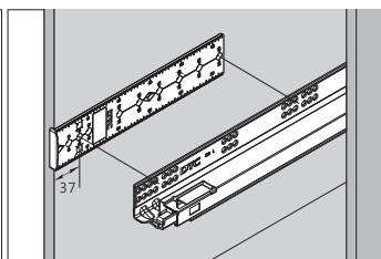
Undermount Slide Series
