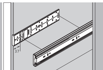
Ball Bearing Slide Series
